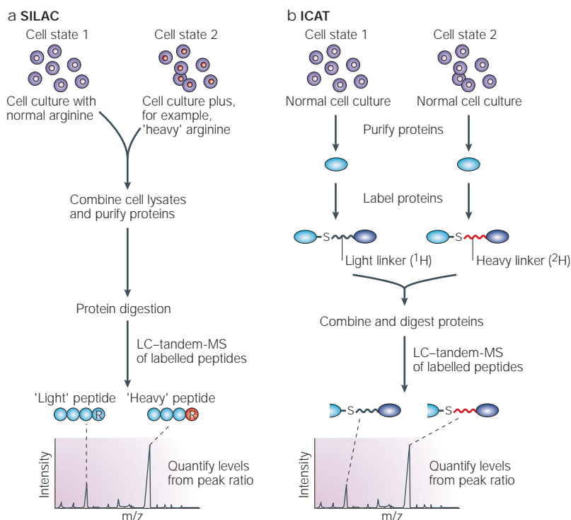
Figure 4 | Techniques for the relative quantification of protein populations. a | A schematic representation of the SILAC ('stable-isotope labelling in cell culture') method. A stably labelled amino acid in a cell-culture medium (in this case, 'heavy' arginine) is incorporated fully into the proteome of one cell population. Relative quantification experiments can easily be carried out using cells that were grown in normal media as the control state. Cell lysates from two conditions can be combined and purified through any number of steps. The proteins are then digested and if the two forms of the peptides co-elute, a peptide ratio can be obtained for each mass spectrum, which allows the protein levels in the two populations to be relatively quantified. b | The ICAT ('isotope-coded affinity tag') method involves the use of a label that is composed of three modular parts — an isotopically labelled linker between a biotin group and a cysteine reactant. Two different isotopically labelled linkers can be used to allow the peptides of two different protein populations from two different cell states to be relatively quantified. The biotin group allows the selective capture and analysis of only the subset of peptides that contain a cysteine residue. LC-tandem-MS, liquid-chromatography-tandem-mass-spectrometry; m/z, mass-to-charge ratio.
