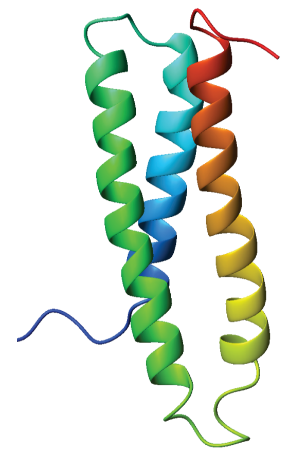
Protein Folding
